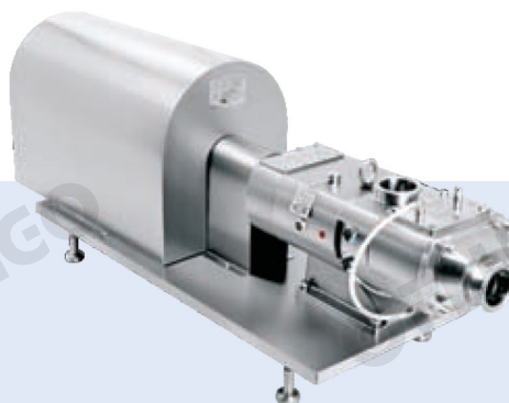
Screw pump with motor cover + Pump head insulation jacket
