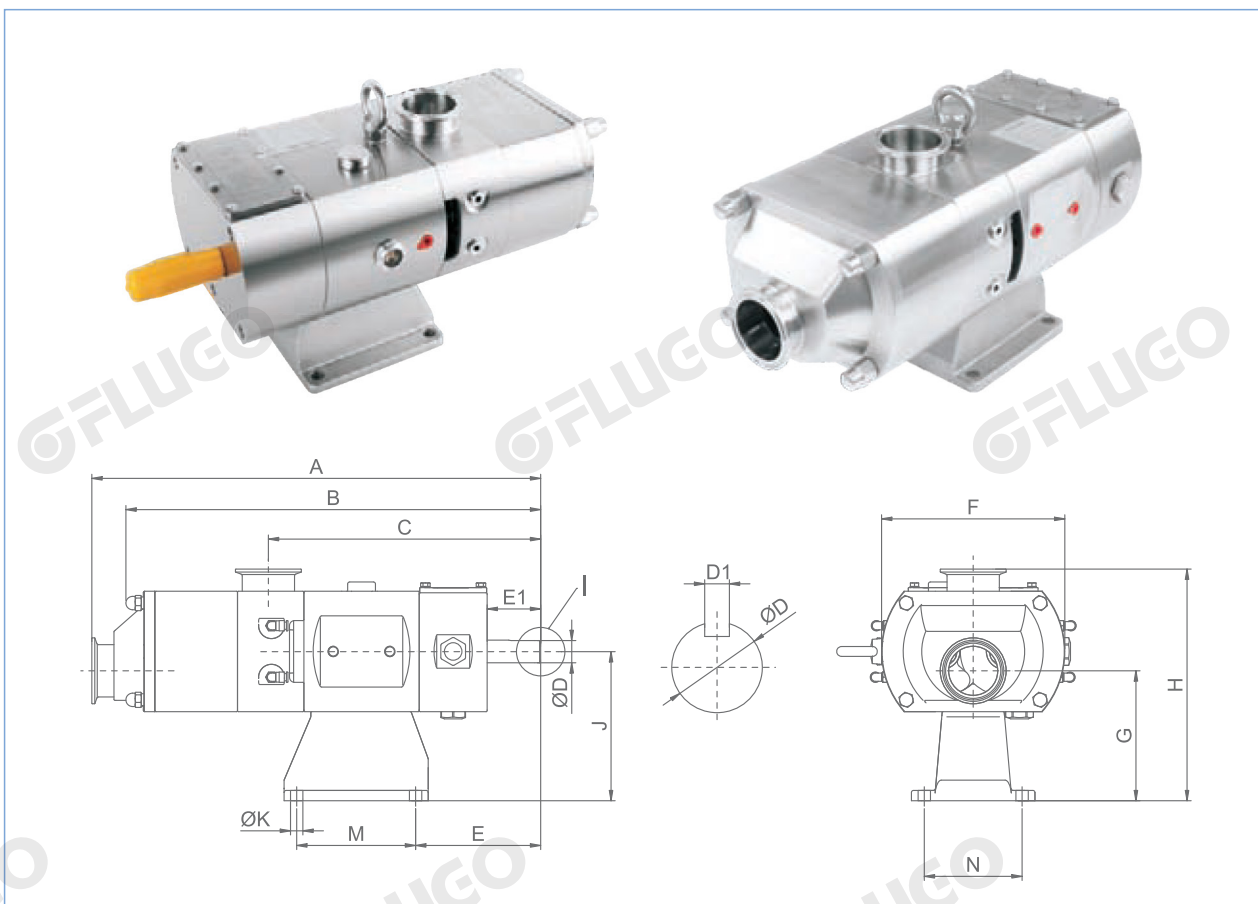
FLG Screw Pump Dimension Data Chart
